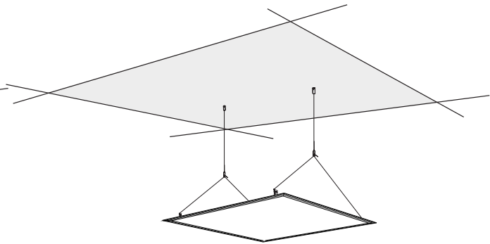
Suspension Installation
